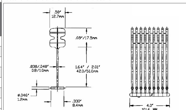
Fastener dimensions for 08390-1 thru 08393-1
