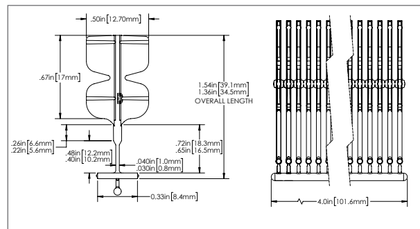
Fastener dimensions for 11243-0 thru 11246-0
